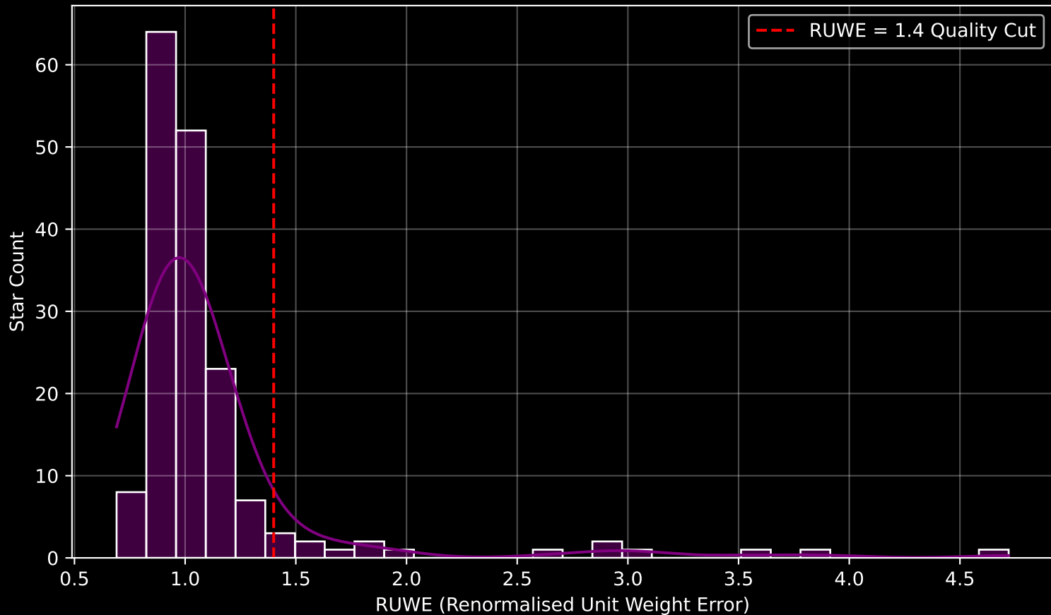
GAPOGEE DR17 Field [CVZTILE_092+20_btx] RUWE Distribution (n= 170)
