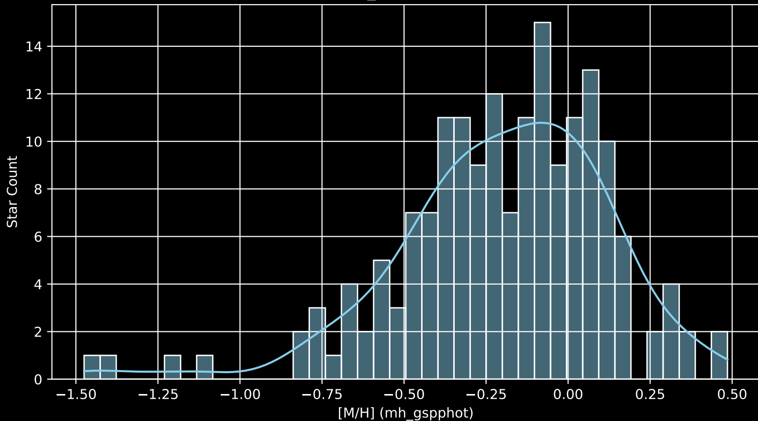
APOGEE DR17 Field: [CVZTILE_092+20_btx [M/H] (mh_gspphot) (n= 173)
