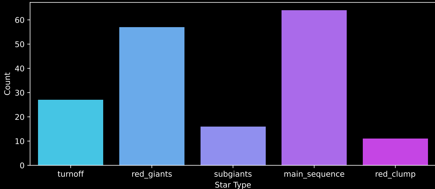
APOGEE DR17 Field: [CVZTILE_092+20_btx] Count plot of Star Type
