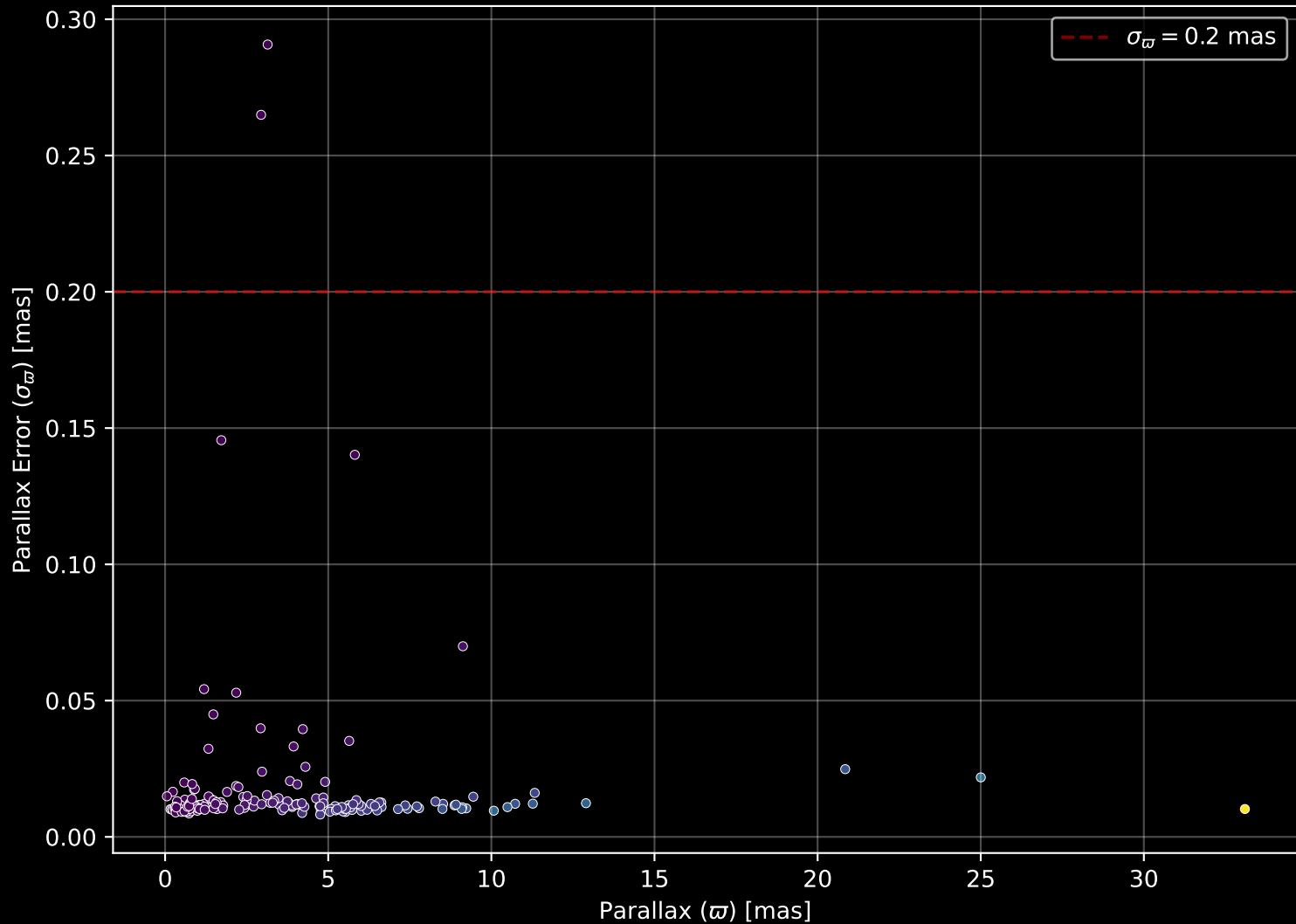
APOGEE DR17 Field: [CVZTILE_092+20_btx] Parallax Quality (n= 175)
