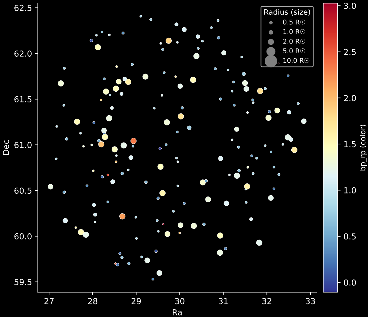
APOGEE DR17 Field: [CVZTILE_092+20_btx] Stars: 175
