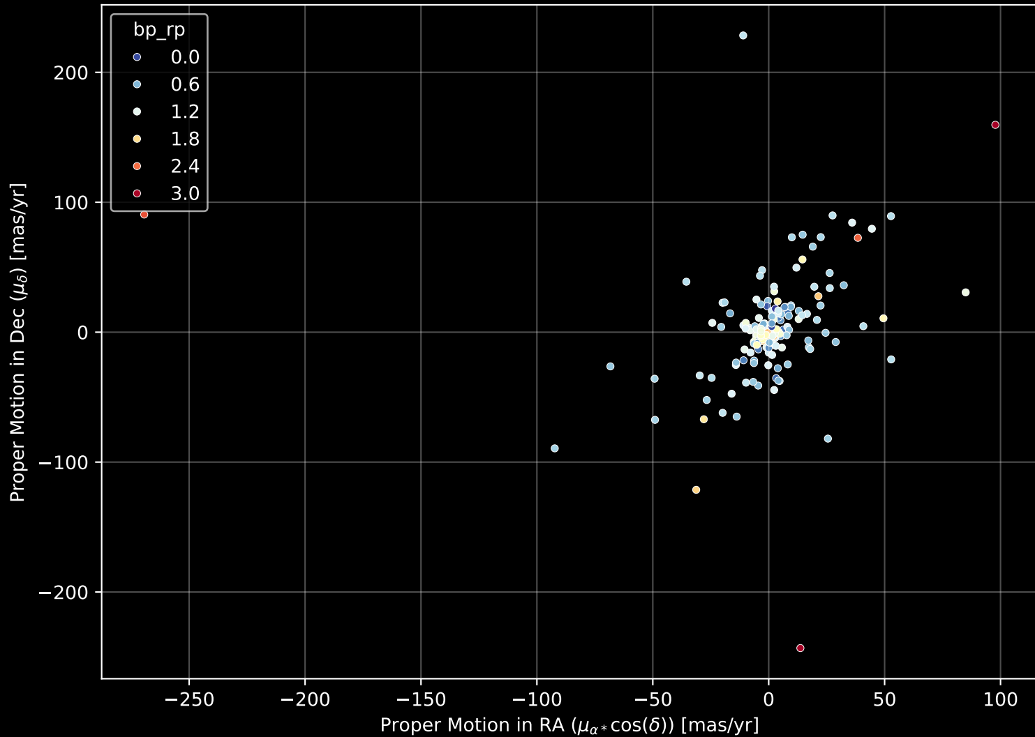
APOGEE DR17 Field: [CVZTILE_092+20_btx] Proper Motion Diagram (n= 175)
